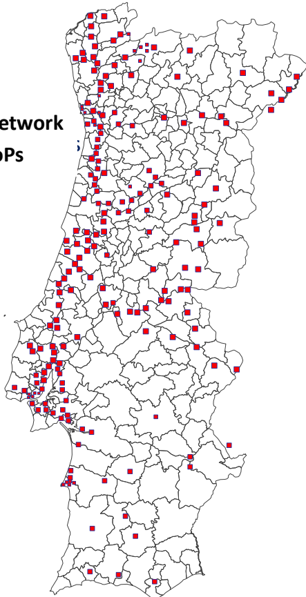
SDH/DWDM network 110 PoPs
